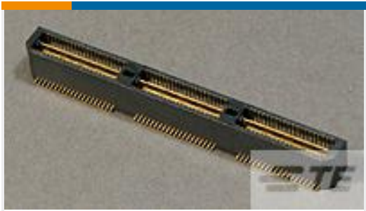
TE Part # 7-1658045-3 MSB0.80PL8ASY84DP,GP,F,VCTR
